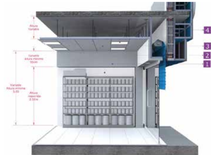
Detalle 1 Cajillo perimetral
